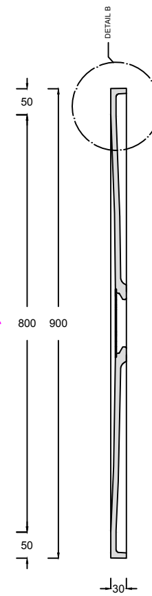
SECTION B:B
