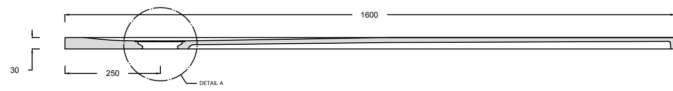
PLAN VIEW
