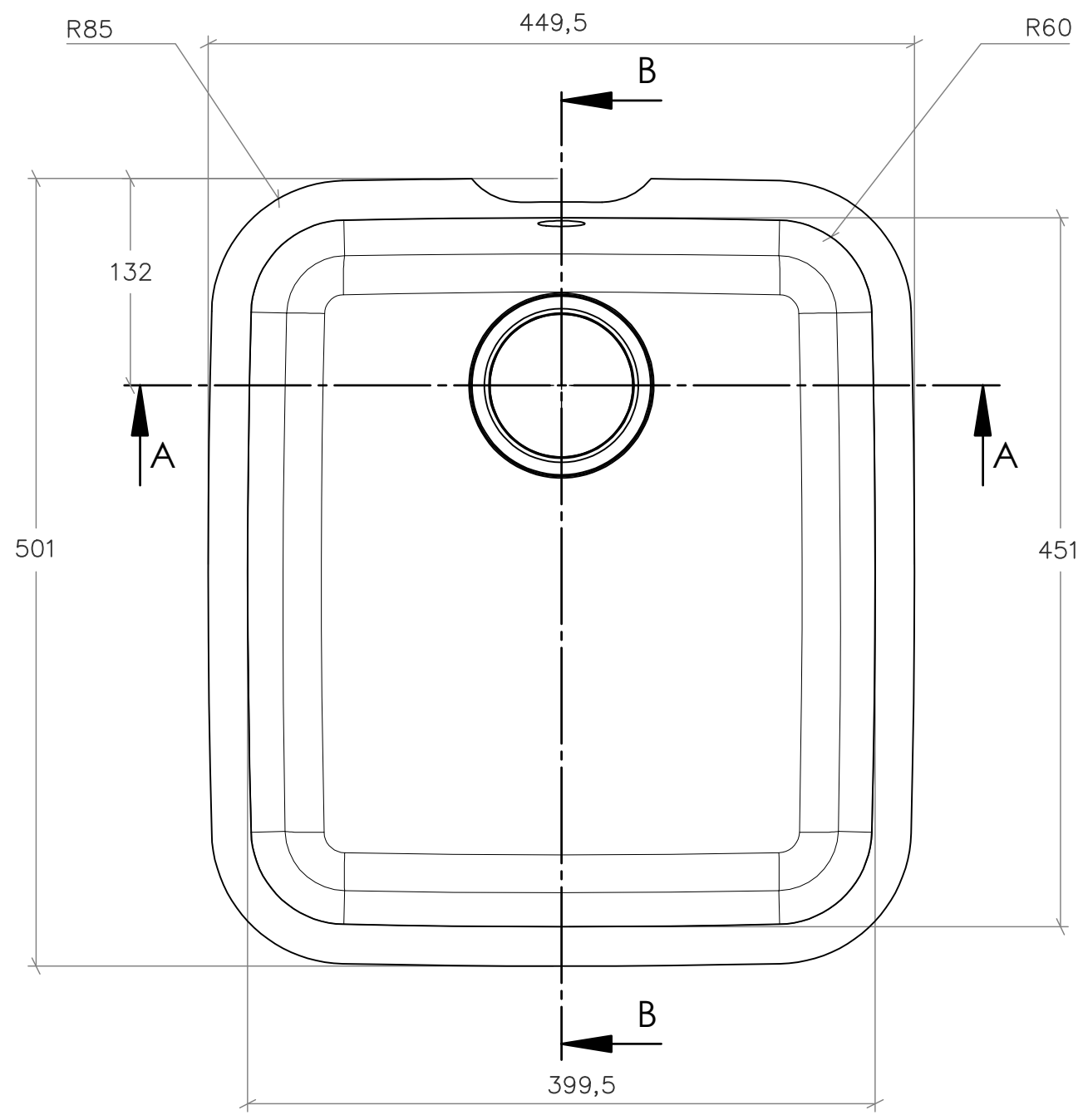
TOP VIEW
